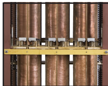
Inner view of Regulator with Carbon Roller Assembly
